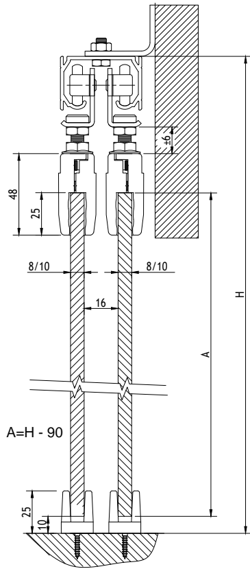
Wall Mounting:
