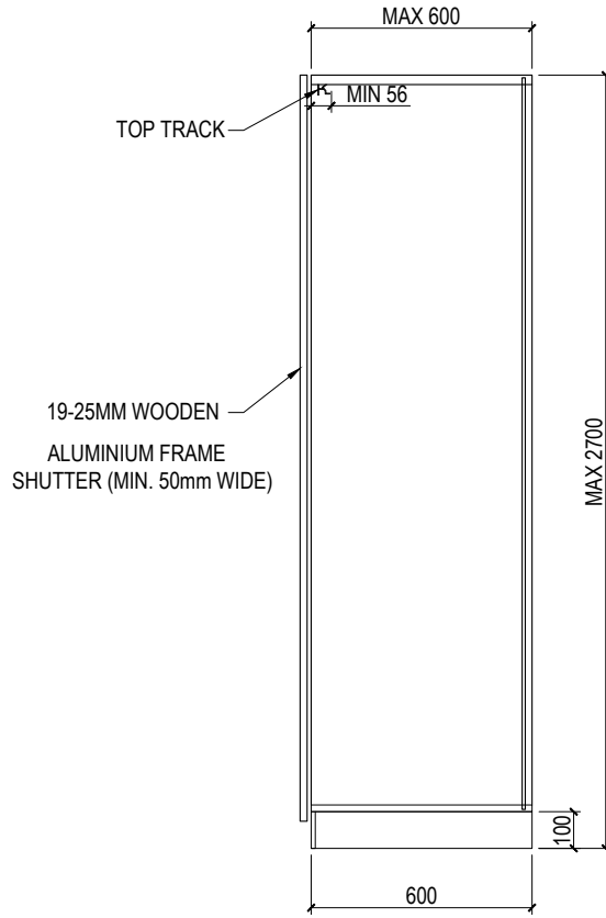
SECTION
