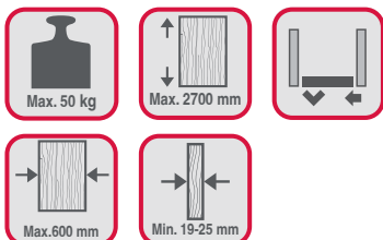
Slide Fold 50
