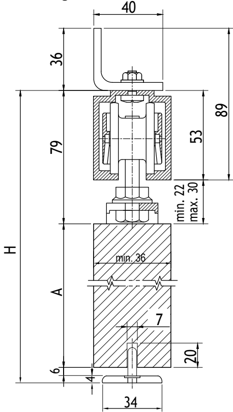
Section View: Wall Mounting
