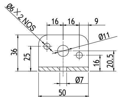
Mounting Bracket:
