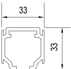
Track Dimension:
