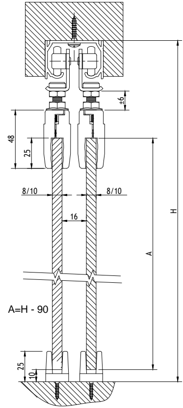
Concealed Mounting:
