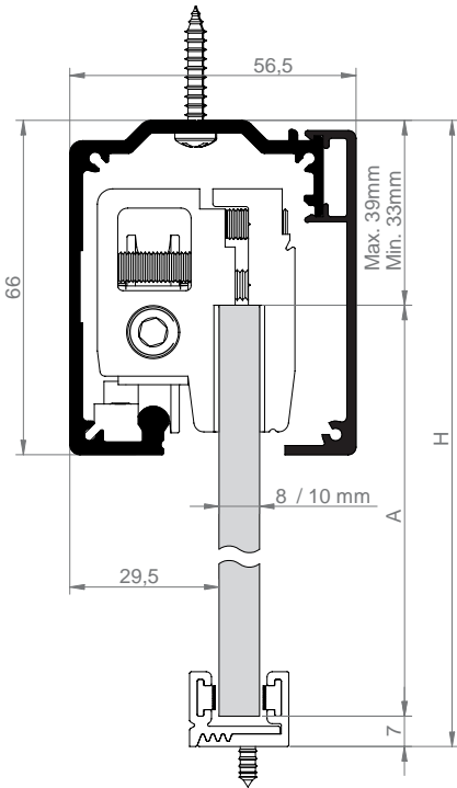
Application - 1 One Sliding Door Ceiling Mounting
