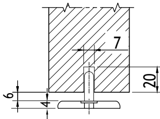
Bottom Guide Cross Section:
