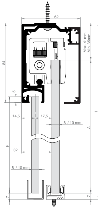
Application - 2 One Sliding Door + One Fixed Panel Ceiling Mounting
