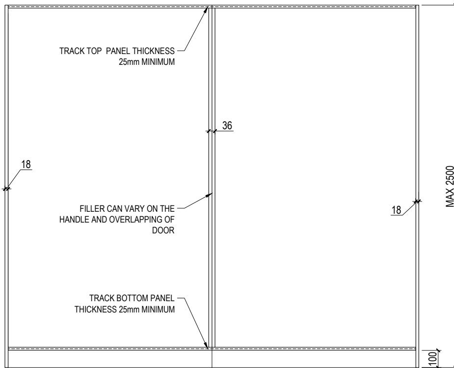
INTERNAL ELEVATION
