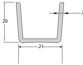
Polypropylene Track
