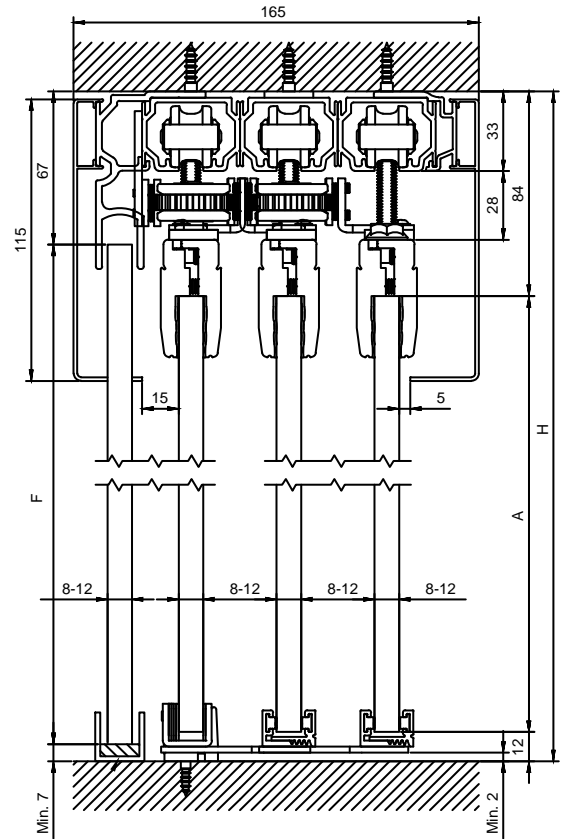
A = H-96
