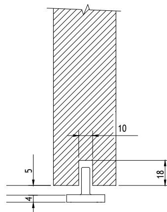
Bottom Guide Cross Section:
