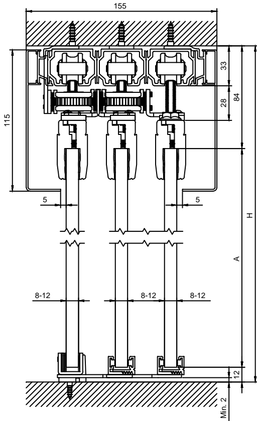
A = H-96
