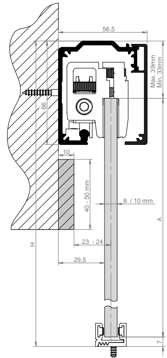
Application - 3 One Sliding Door Wall Mounting
