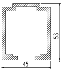
Track Dimension:
